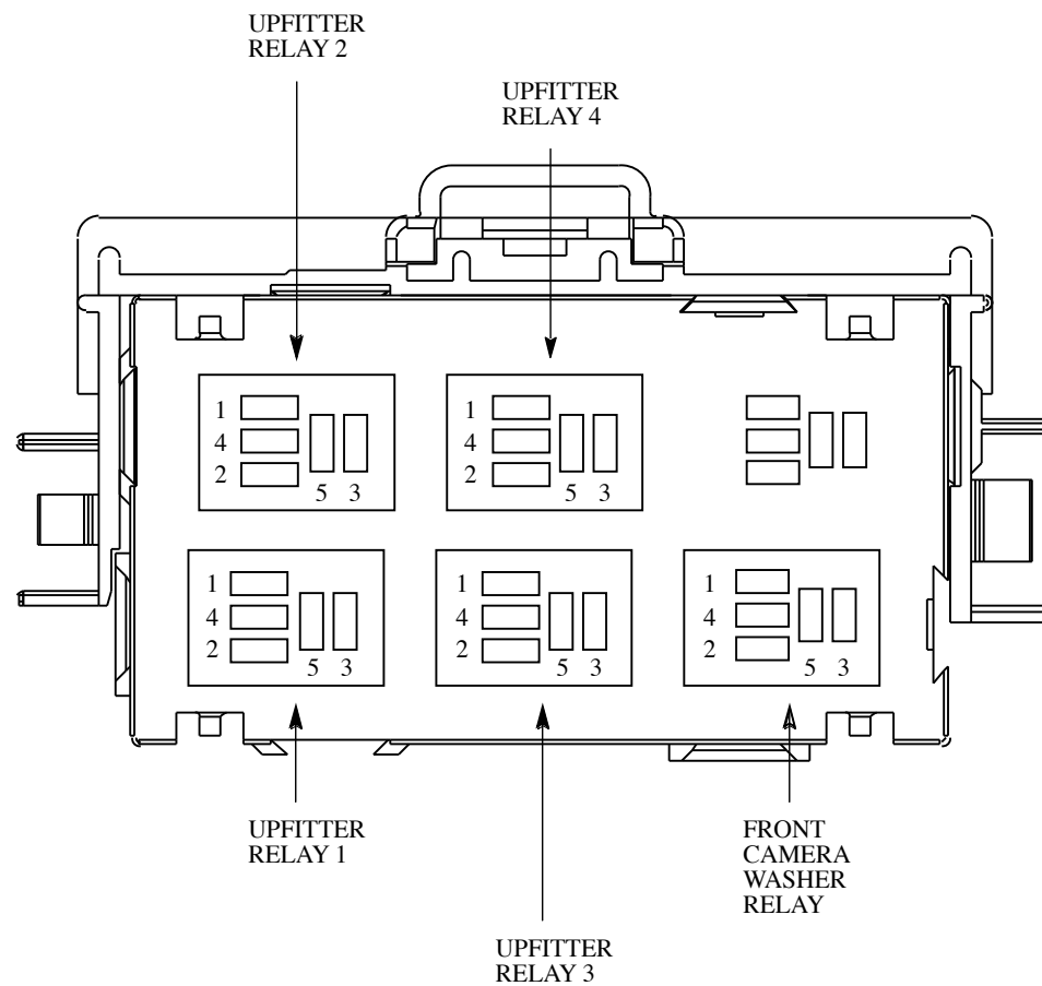
AUXILIARY BATTERY JUNCTION BOX (BJB)
